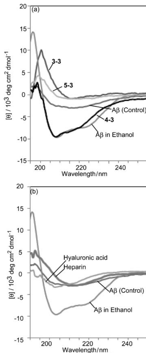
Figure 4. CD spectra of A \beta (1–40). The A \beta solution was prepared by the incubation of A \beta (46 \mu M) at pH 7.5 and 37 ^{\circ} C with 400 rpm shaking for 48 h. The CD spectra were (a) in the presence of glycopolymers of 3-3 , 4-3 , and 5-3 at 400 \mu M, and (b) in the presence of polysaccharide of hyaluronic acid and heparin at 1.0 mg mL −1 .
