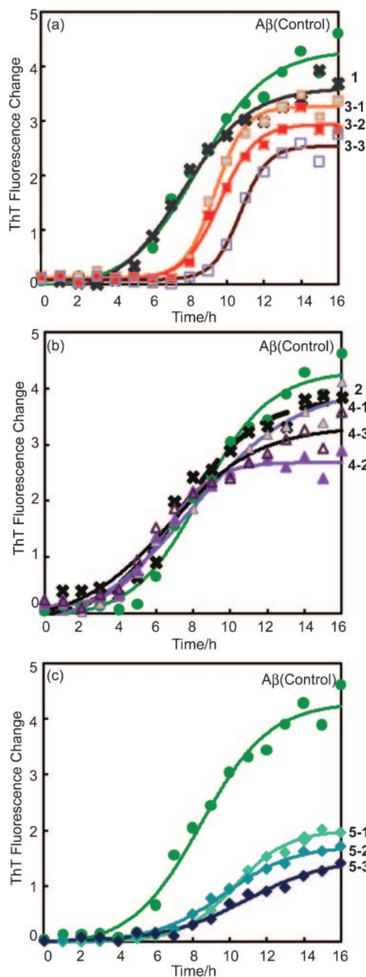
Figure 2. Time course of fibril formation at pH 7.5 and 37°C with 400rpm shaking monitored by ThT fluorescence. The concentrations of A \beta and sugar were 23 and 200 \mu M, respectively. The sugar additives were (a) poly(acrylamide/6-sulfo-GlcNAc), (b) poly(acrylamide/GlcA), and (c) poly(acrylamide/GlcA/6-sulfo-GlcNAc).
